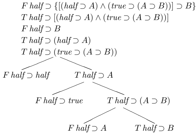
Figure 2: A Non-Modal Proof in \mathcal{T}(3)
